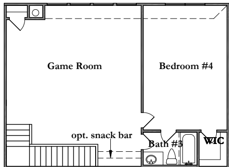
Optional Game Room with Bedroom #4
