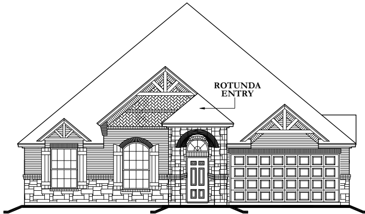
Old World Elevation
