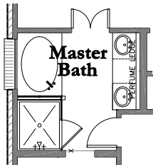
Optional Master Bath Perfume Ledge
