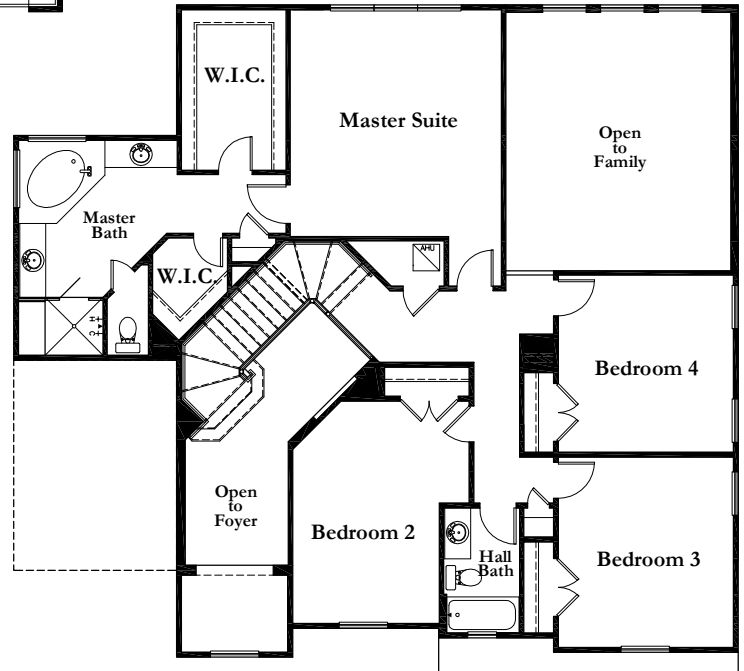
Second Floor
